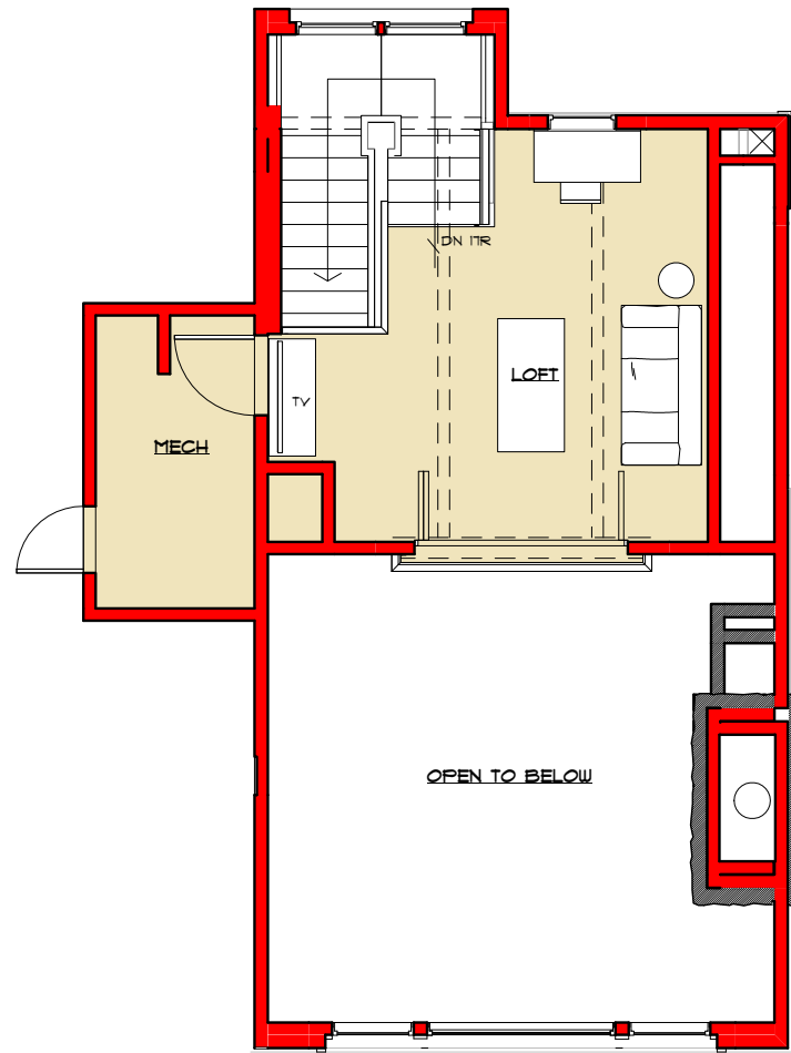
LOFT LEVEL PLAN.
